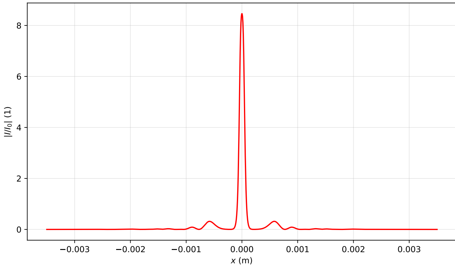
Intensity profile I(x, y = 0, z = 0.478)/I_0 , P_{in}=8.0P_{cr} , artificial time
